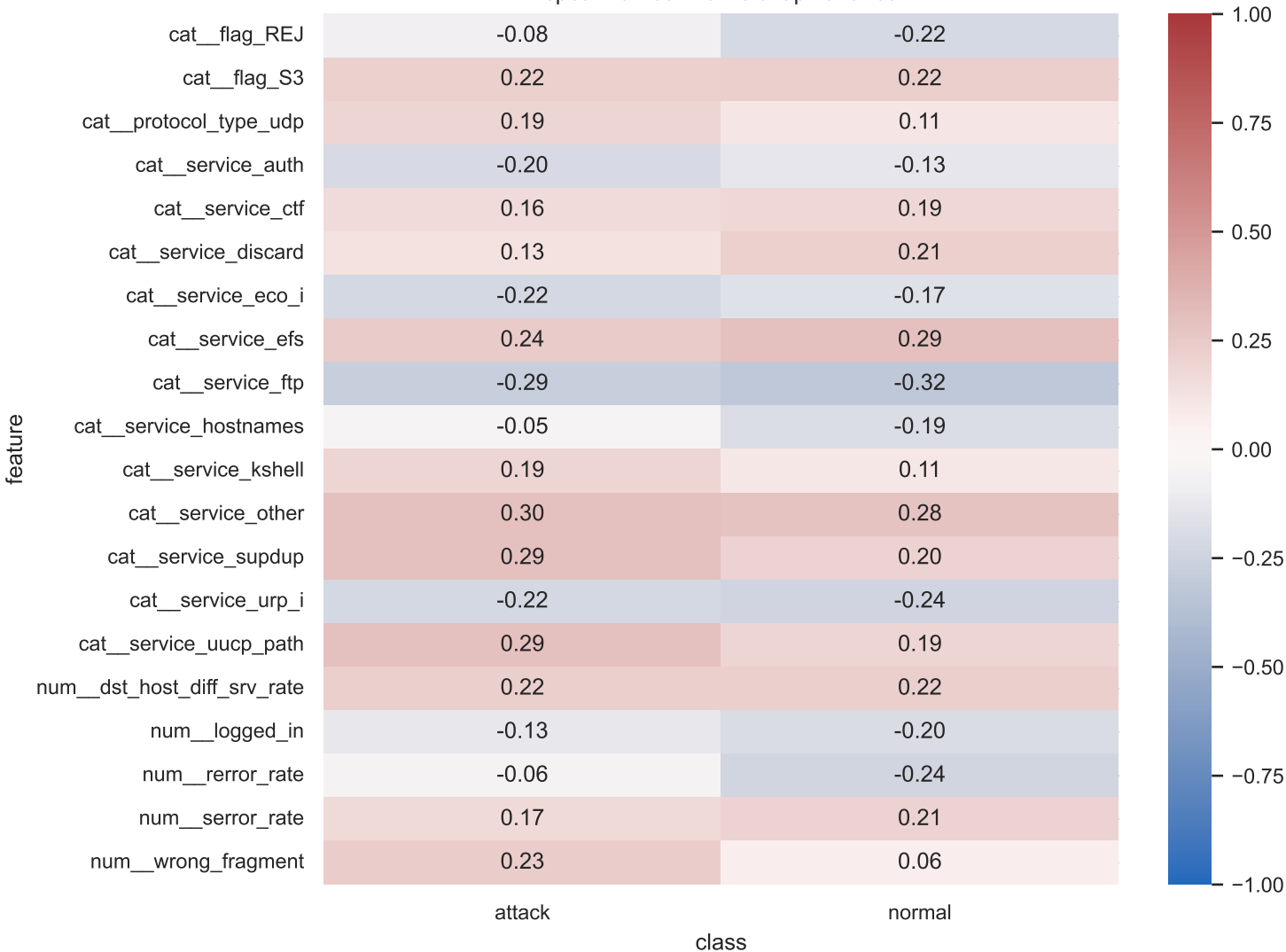
spearman conflict vs shap variance
